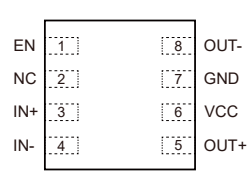
DFN2x2-8L
