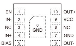
DFN3x3-10L
