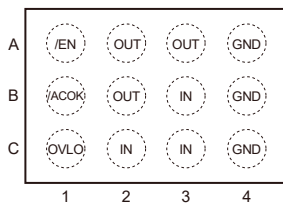
QFNFC1.8x1.3-12L
