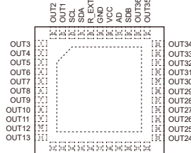
QFN5x5-44L
