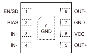
DFN3x3-8L/DFN2x2-8L
