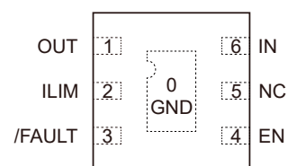
TDFN2x2-6L
